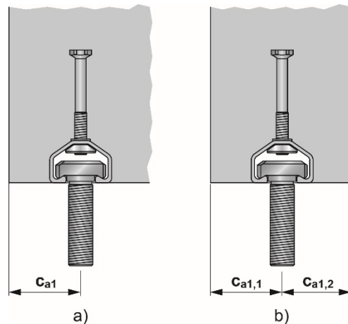
Figure 4-9: Anchor channel
