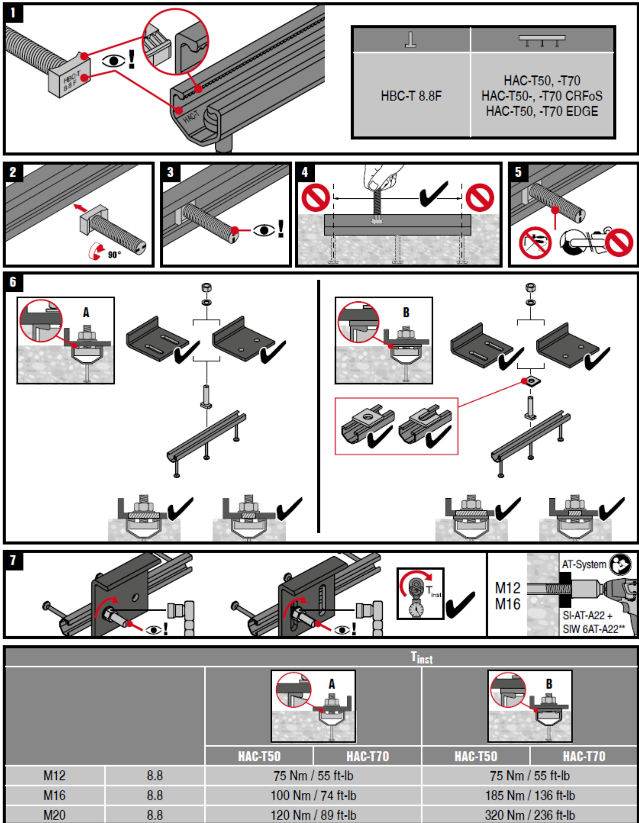
FIGURE 8-9: MANUFACTURER'S PRINTED INSTALLATION INSTRUCTIONS (MPII) FOR HILTI CHANNELS BOLTS (HBC-T)
