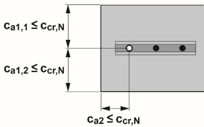
b) anchor channel with influence of two edges and one corner
