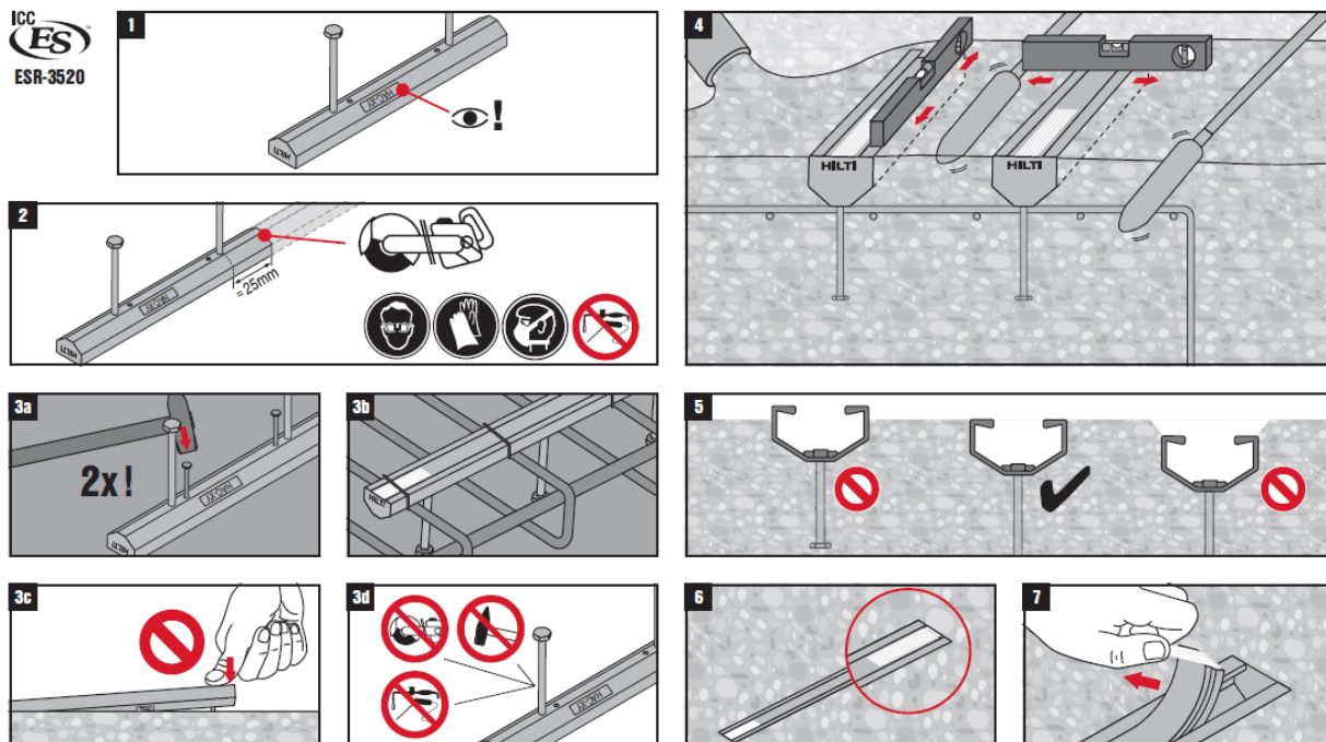
FIGURE 8-6: MANUFACTURER'S PRINTED INSTALLATION INSTRUCTIONS (MPII) FOR HILTI ANCHOR CHANNELS (HAC AND HAC-T)
