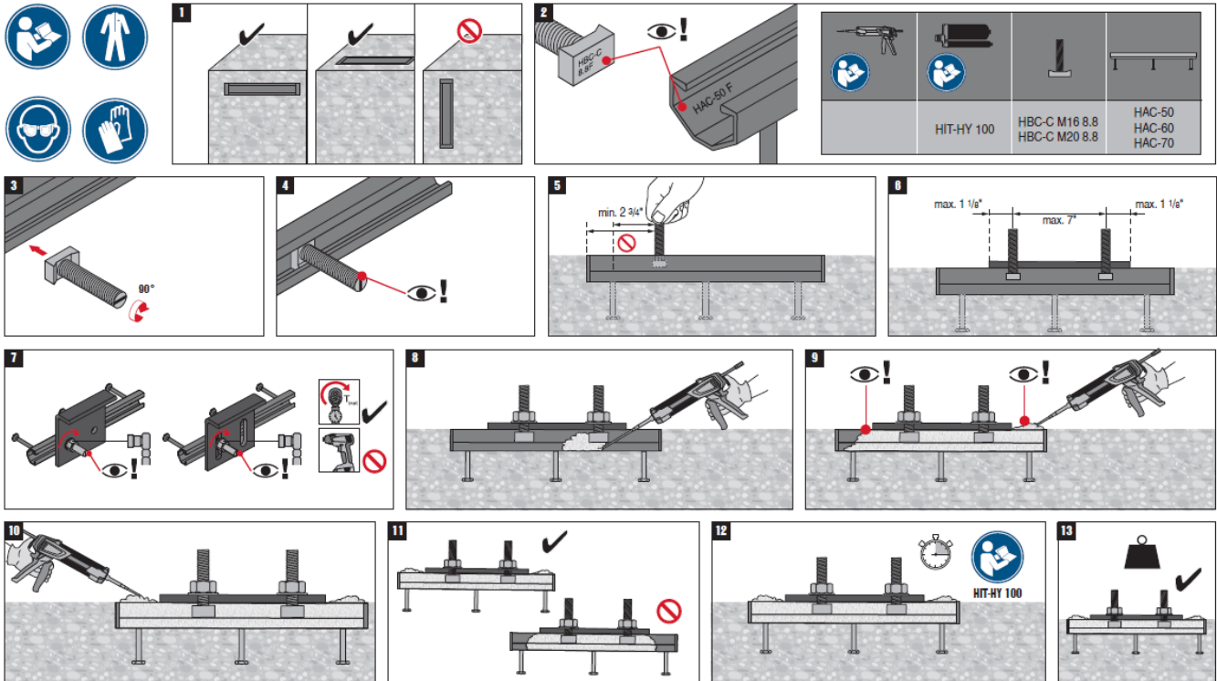
FIGURE 8-11: MANUFACTURER'S PRINTED INSTALLATION INSTRUCTIONS (MPII) FOR HILTI ANCHOR CHANNELS (HAC) WITH HILTI CHANNEL BOLTS (HBC-C) USED IN CONJUNCTION WITH HILTI HIT HY-100 ADHESIVE
