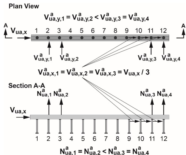
Figure 4-3: Example for the calculation of anchor forces in case of anchor channels with 12 anchors loaded in shear longitudinal to the channel axis for steel and pryout failure
