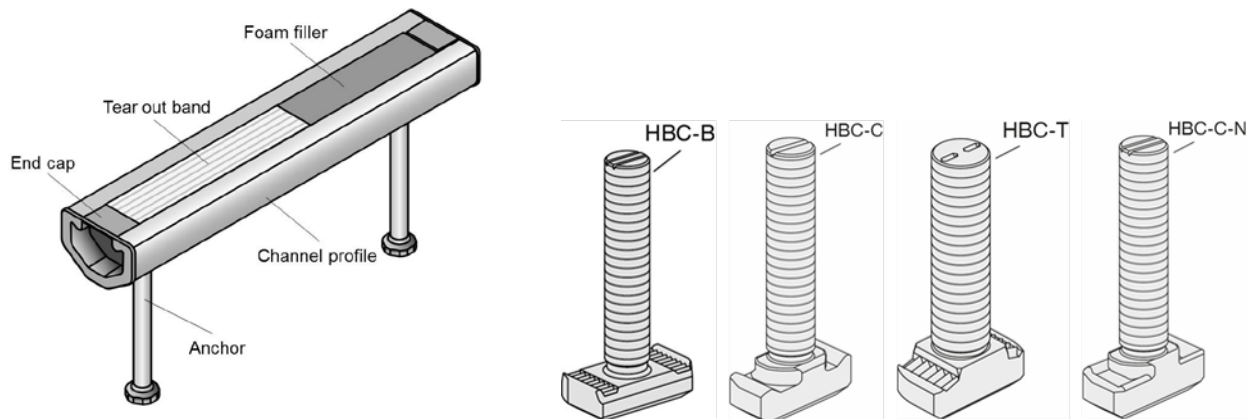
FIGURE 8-3: ANCHOR CHANNELS HAC AND HAC-T AND CHANNEL BOLTS HBC-B, HBC-C, HBC-T AND HBC-C-N
